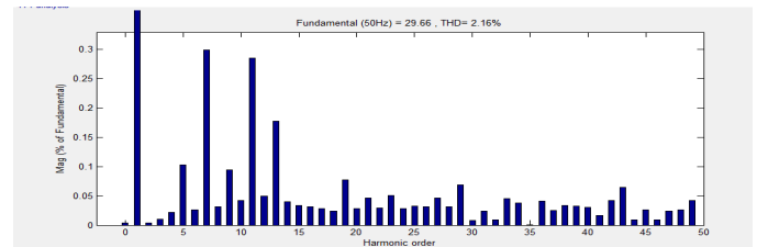
Fig. 10 Harmonics spectrum with PI controller
