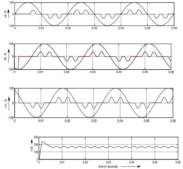
Fig. 8 Waveform without controller
