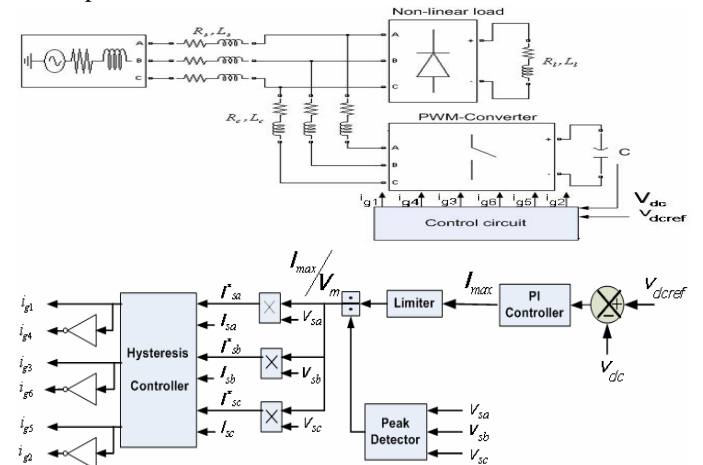
Fig. 2 a) Active filter system b) Active filter system using PI controller
