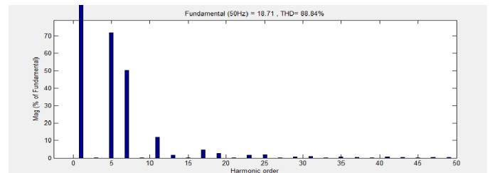
Fig. 9 Harmonics spectrum without controller
