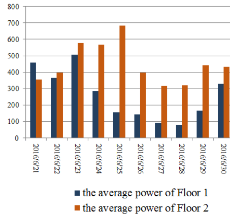
Fig. 10. The prediction results using the proposed online sequential ELM.
