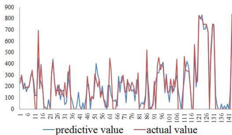
Fig. 8. The power consumption without our system.
