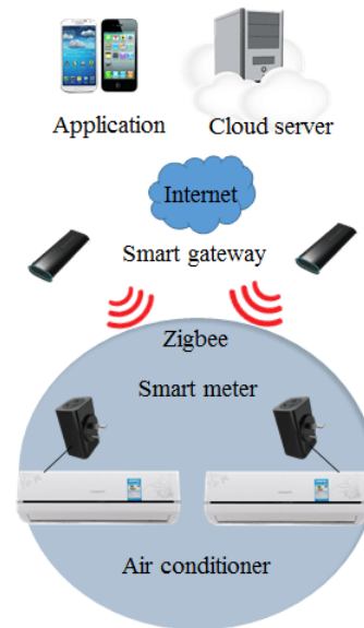
Fig. 3. The Architecture of the developed smart meter.
