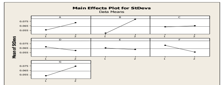
Figure5.3 Response graph of std deviation
