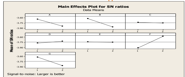
Figure5.1 Response graph of S/N ratio
