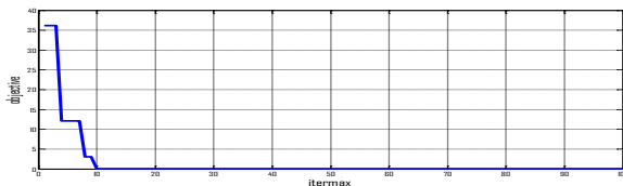
Fig.1 Convergence characteristic of TVAC PSO for 3 generating units.
