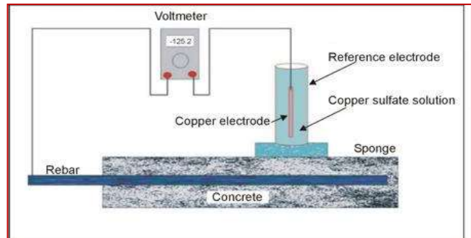
Figure-3 Half Cell Potential Test
